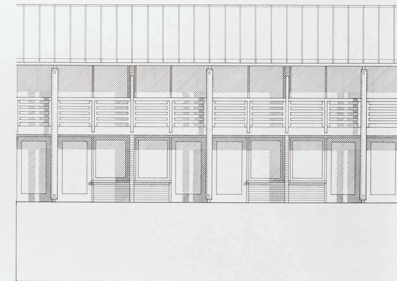
DETAIL ELEVATION 1.50
